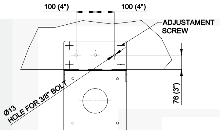
TOP FIXING
