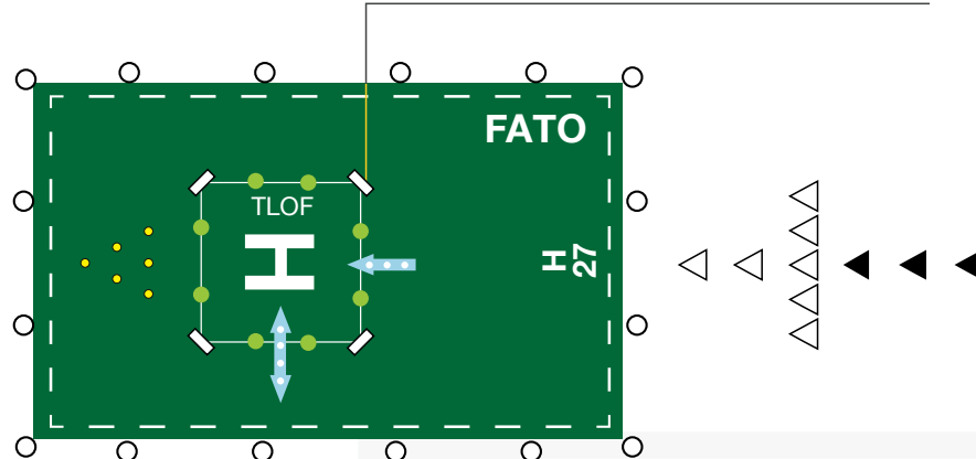
HELIPORT FLOODLIGHT (night) HFL-LXS-10K
