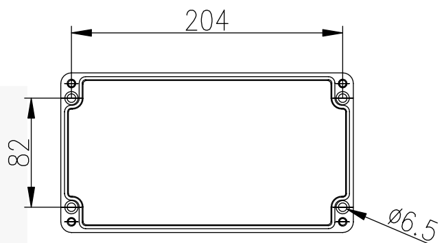
FLIXING DETAILS
