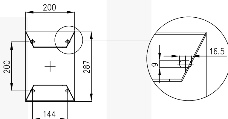
FIXING DETAILS
